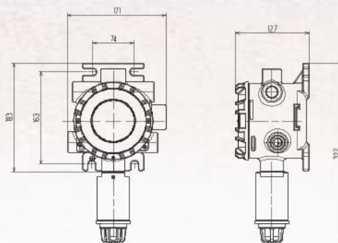
Diffusion type with EC barrier
