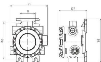
Main unit (SD-3SC)
