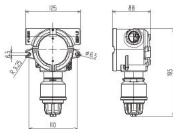
Remote sensor unit (GD-3 Series) Diffusion type without EC barrier
