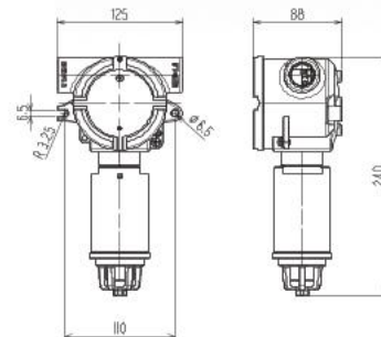
Remote sensor unit (GD-3 Series) Diffusion type with EC barrier
